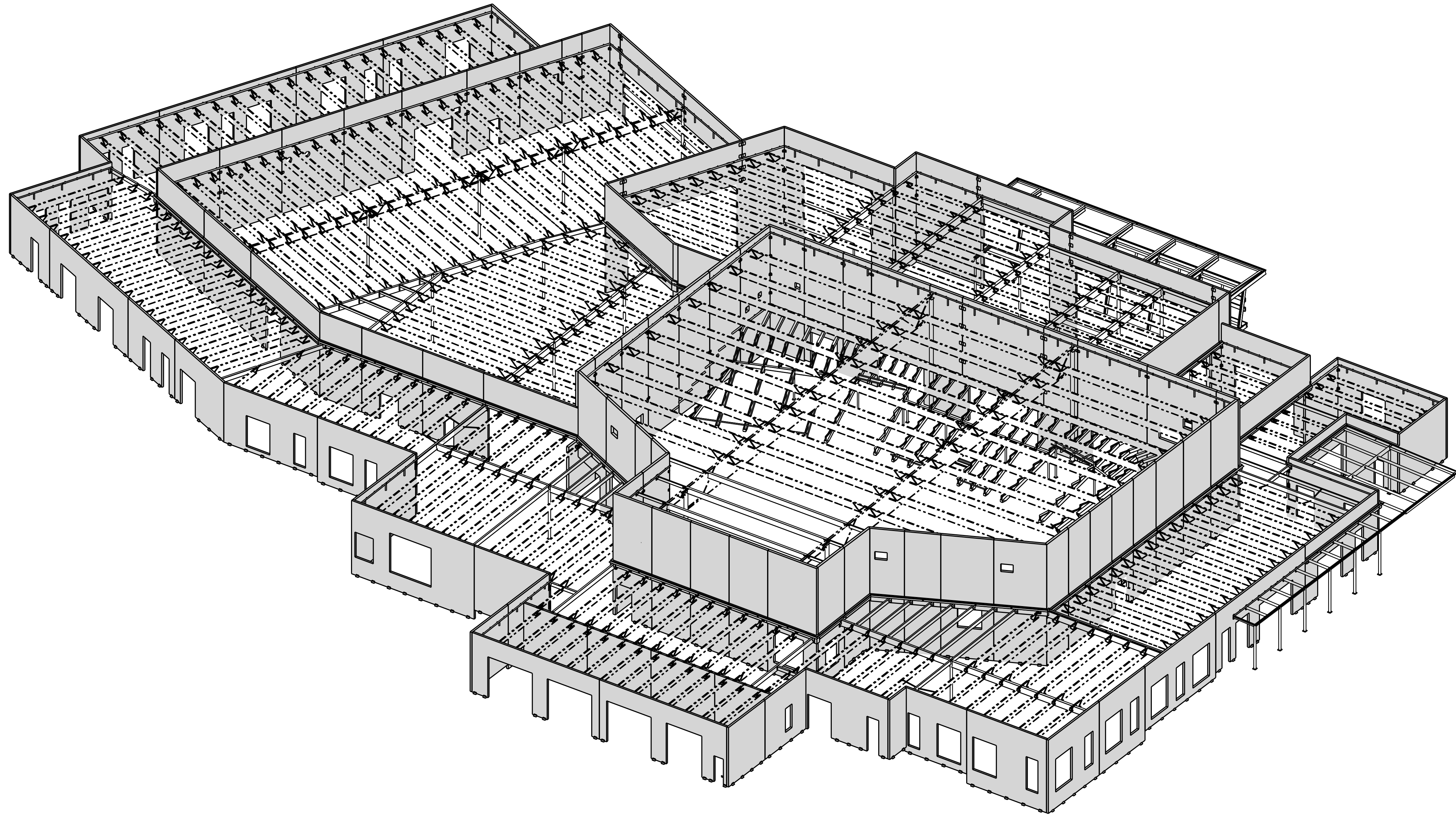
3D - VIEW BETHLEHEM CHURCH MAIN CAMPUS - MAIN BUILDING
