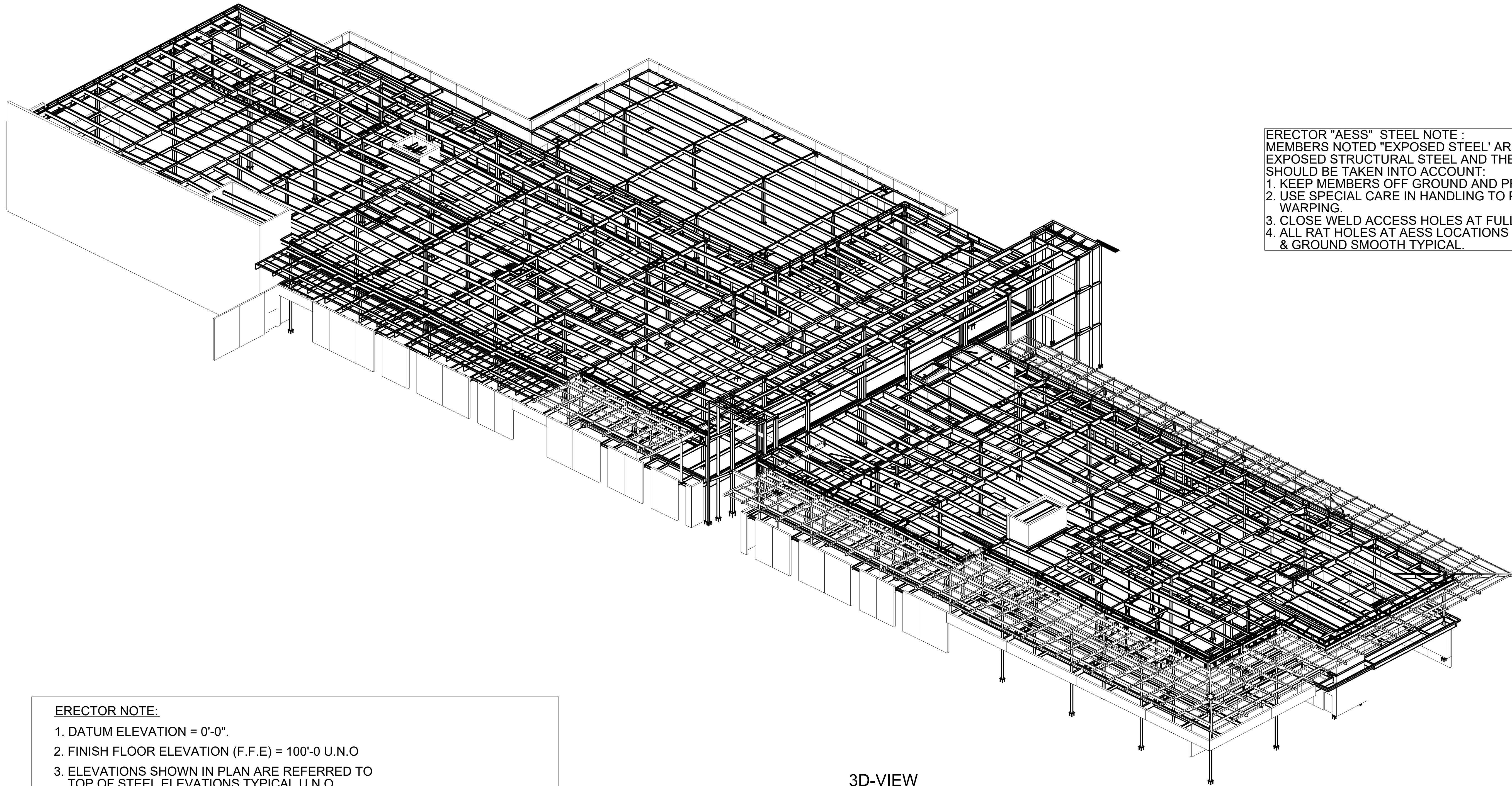
3D-VIEW SOUTH - EAST DIRECTION
