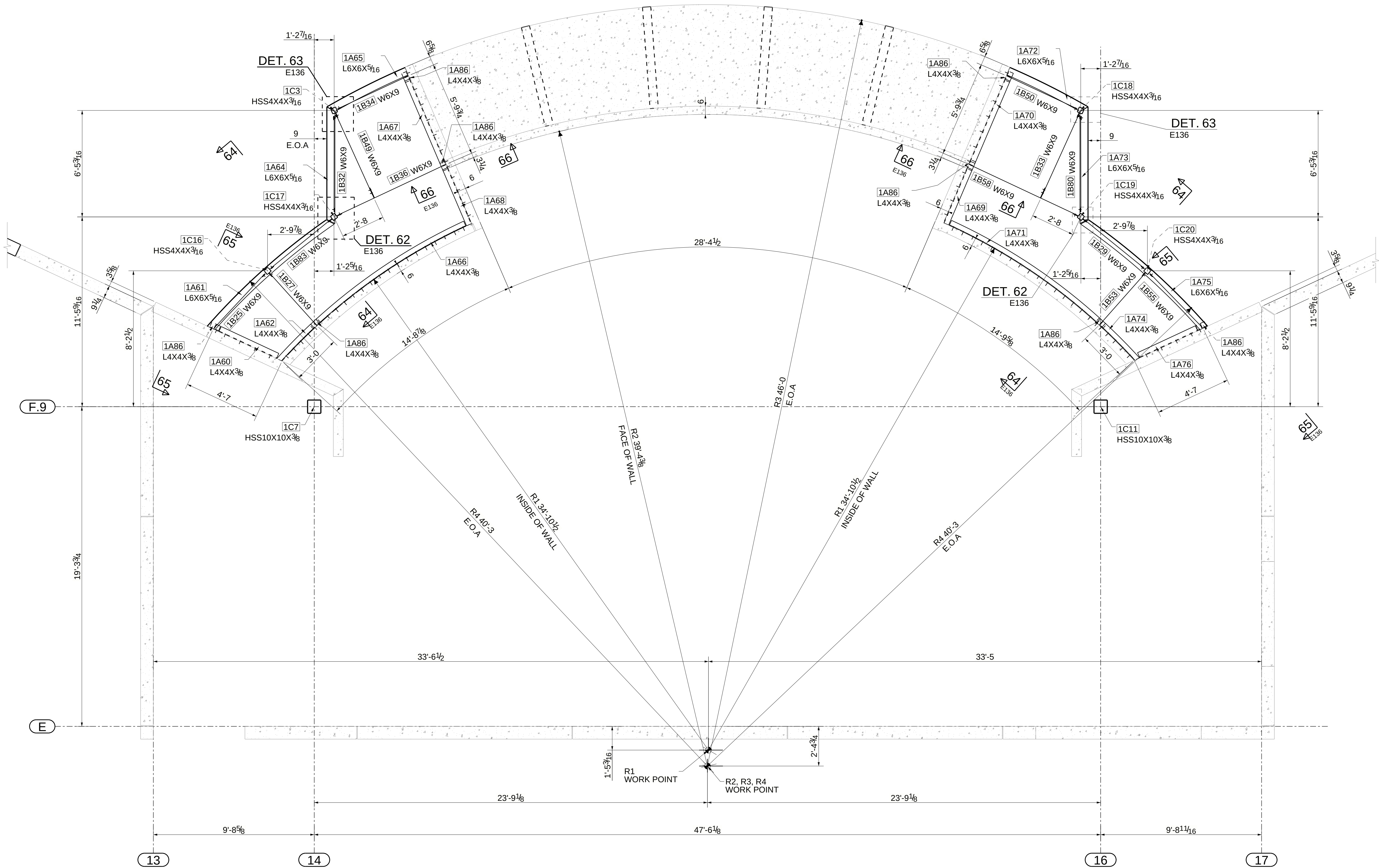
DETAIL P E101 PARTIAL WORSHIP FRAMING PLAN @ TOP OF BEAM ELEVATION = 2'-4 1/2" (REFER : 1/FOUNDATION PLAN - MAIN WORSHIP / S-102)
