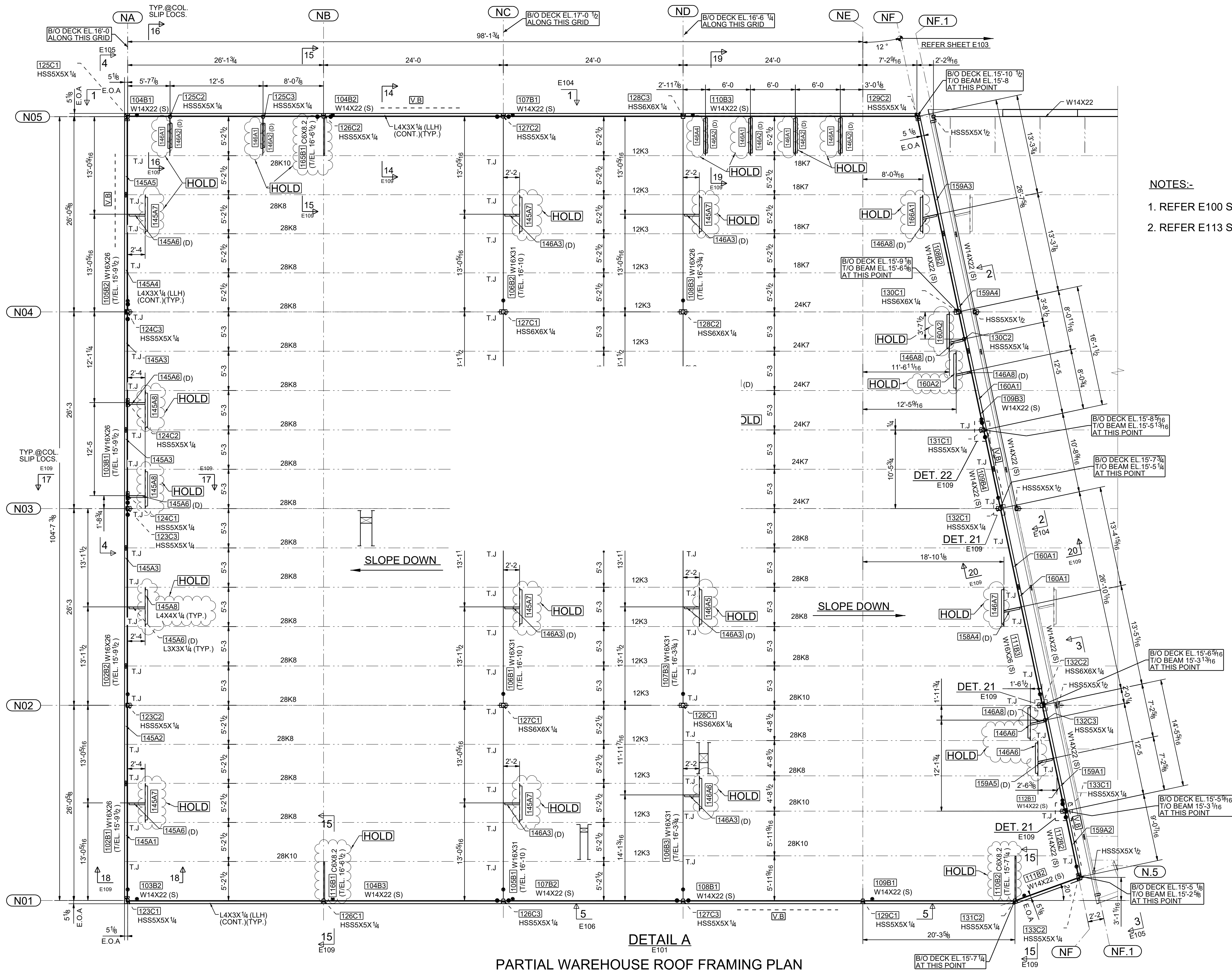
DETAIL A E101 PARTIAL WAREHOUSE ROOF FRAMING PLAN
