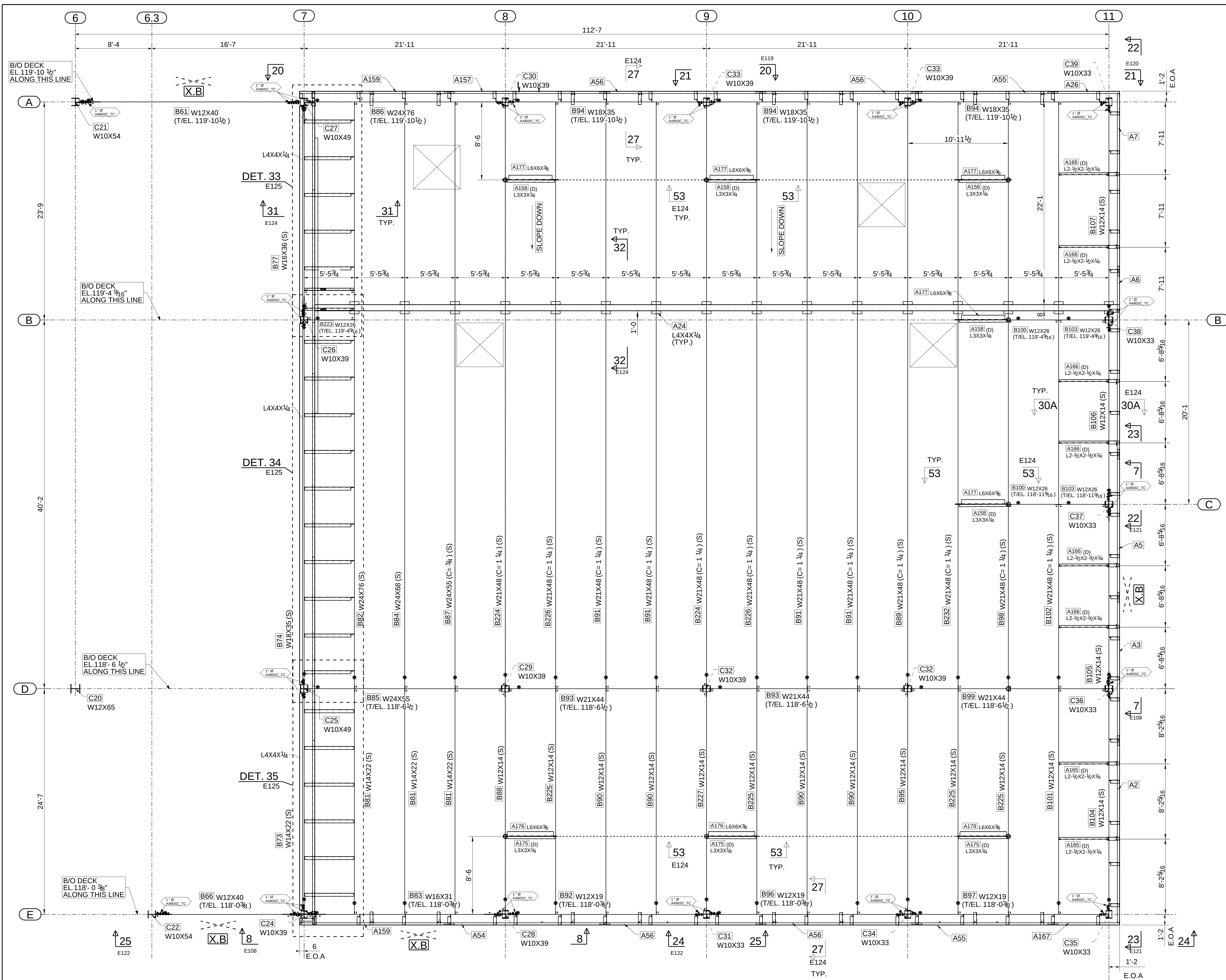
LOW ROOF FRAMING PLAN (REFER : ROOF FRAMING PLAN / 030.A2.94.S.01.30)
